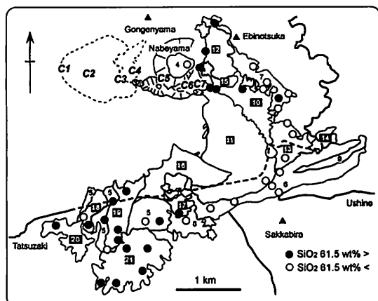
Fig. 14. Map showing spatial distribution of SiO 2 content of the 1914-1915 lava on the eastern flank. Units with simple numbers are T1 lavas, while those with white numbers on a black background belong to T2 and T2' lavas.
