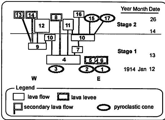
Fig. 4. Diagram showing stratigraphic relationships between units of the 1914 eruptive products on the western flank. Black tie lines between blocks are stratigraphic relations based on the aerial photos. Approximate date is shown on the right.
